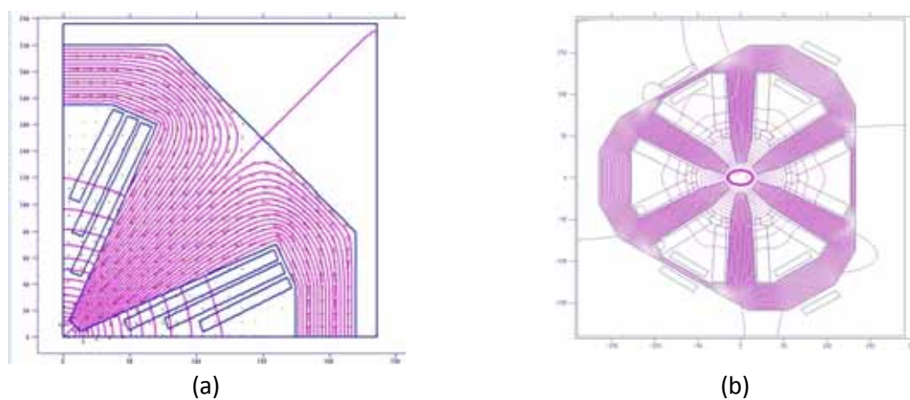
Figure 8: Electro magnets: quadrupoles (a) and sextupoles
